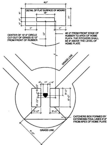
Diagram showing layout of batter's box and compulsory dimensions.
